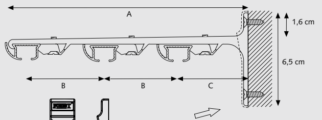
Smart klick cover cap for aluminium wall bracket
